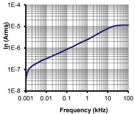
Figure 14: Typical total output current noise (rms) with R_M = 50 \Omega
